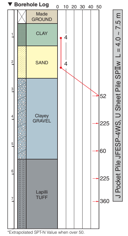
Project : Demolition of Miyagi Prefectural Public Health and Environment Bldg.- Second Phase Location : Sendai City, Miyagi Period : October 2013 ~ November 2013 Silent Piler : F201 Type of Sheet Pile : J Pocket Pile JFESP-4WS, U Sheet Pile SP IIw Pile Length : 4.0 ~ 7.5 m
